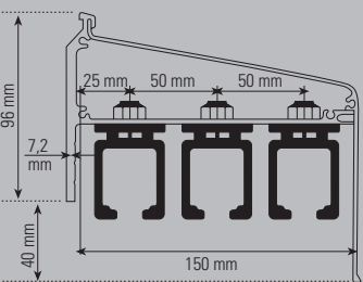
Profilkit 3-spurig
